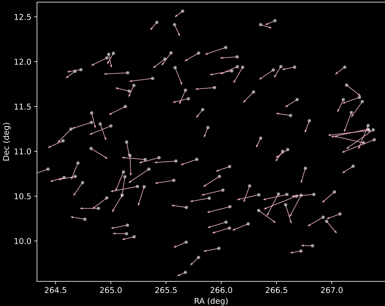
APOGEE DR17 Cluster 13 Proper Motion Vectors (n=112)
