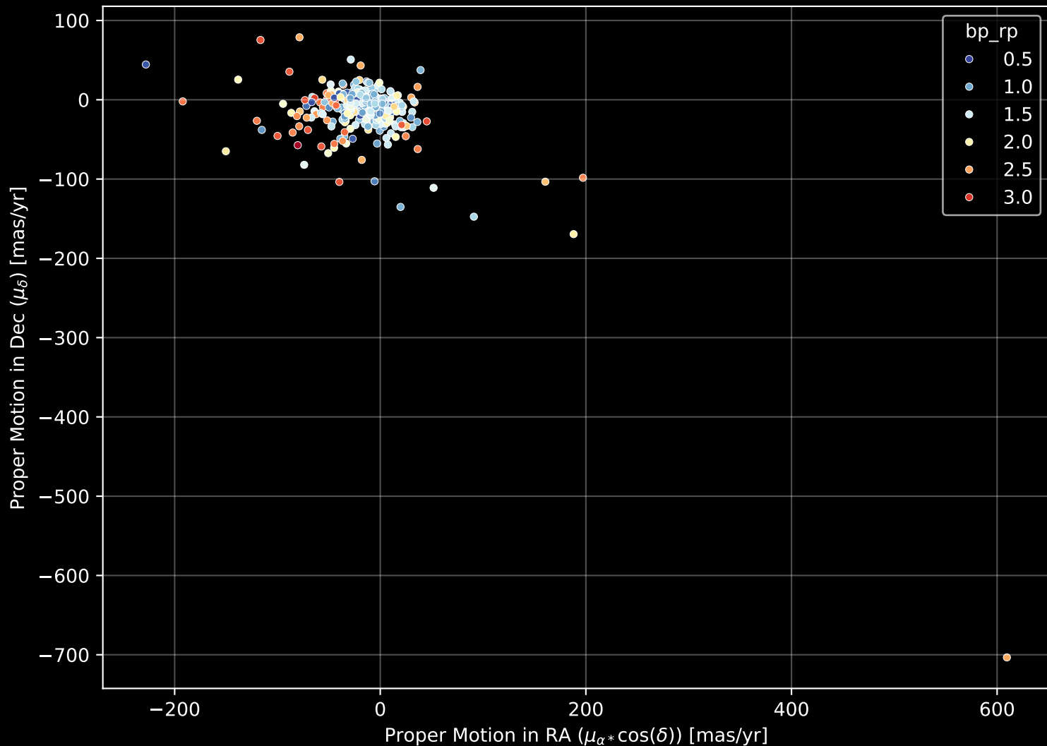
APOGEE DR17 Field: [240+60] Proper Motion Diagram (n= 450)
