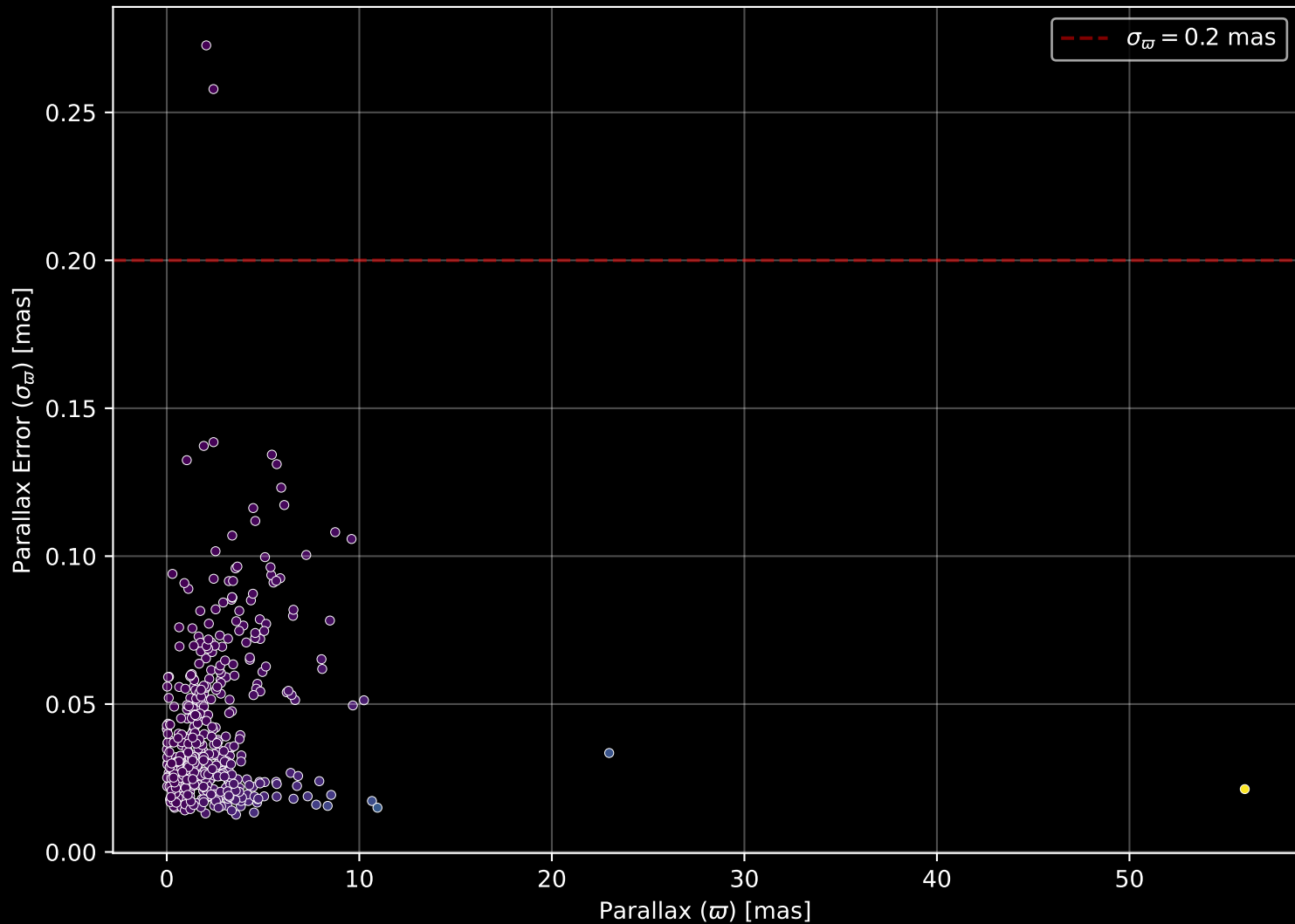
APOGEE DR17 Field: [240+60] Parallax Quality (n= 450)
