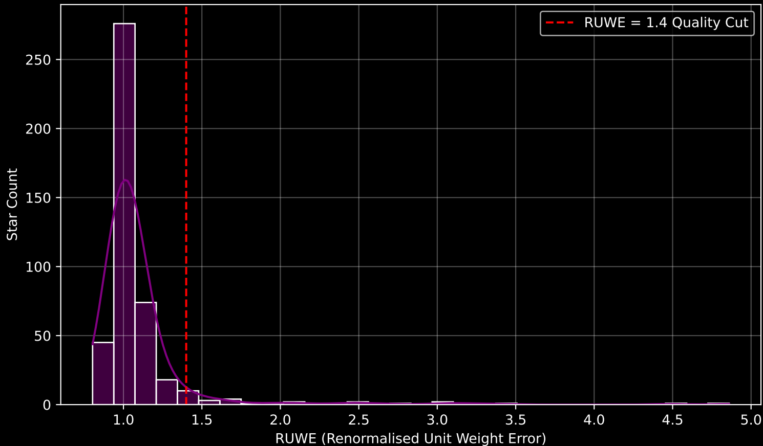
GAPOGEE DR17 Field [240+60] RUWE Distribution (n= 444)
