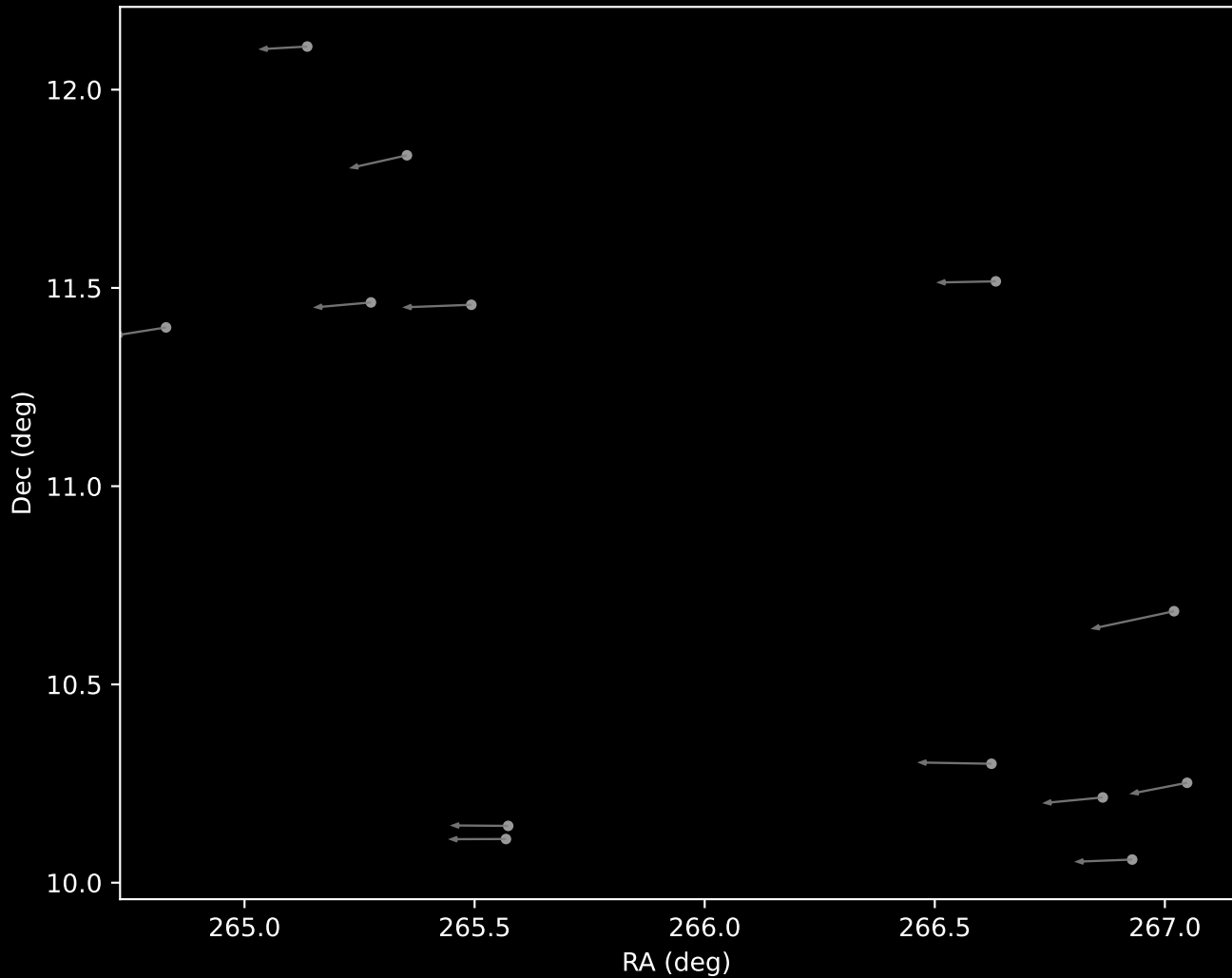
APOGEE DR17 Cluster 14 Proper Motion Vectors (n=13)
