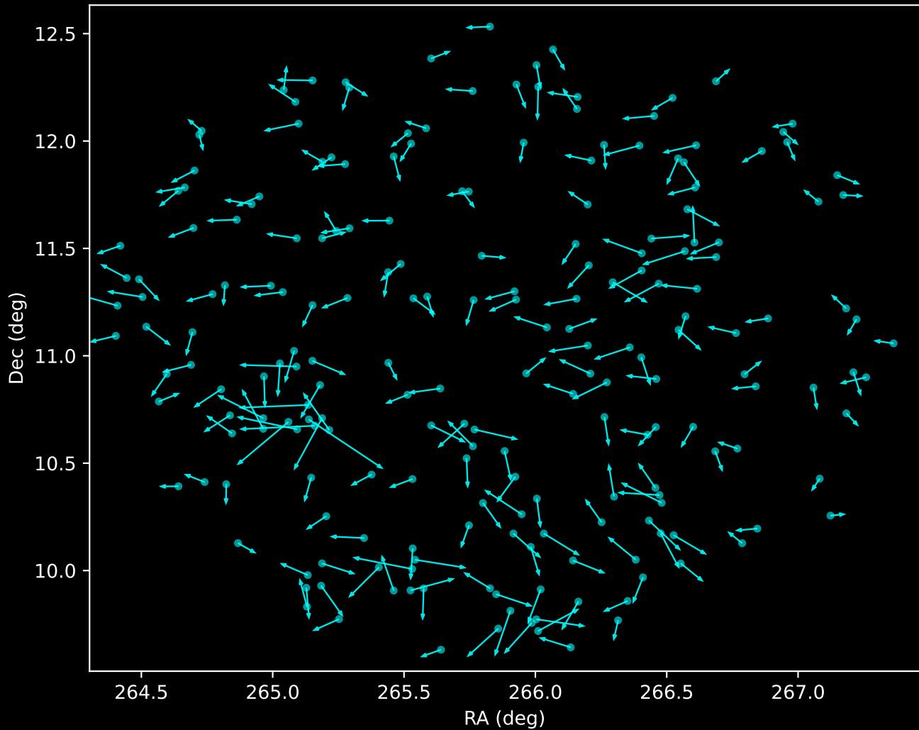
APOGEE DR17 Noise Stream Proper Motion Vectors (n=211)
