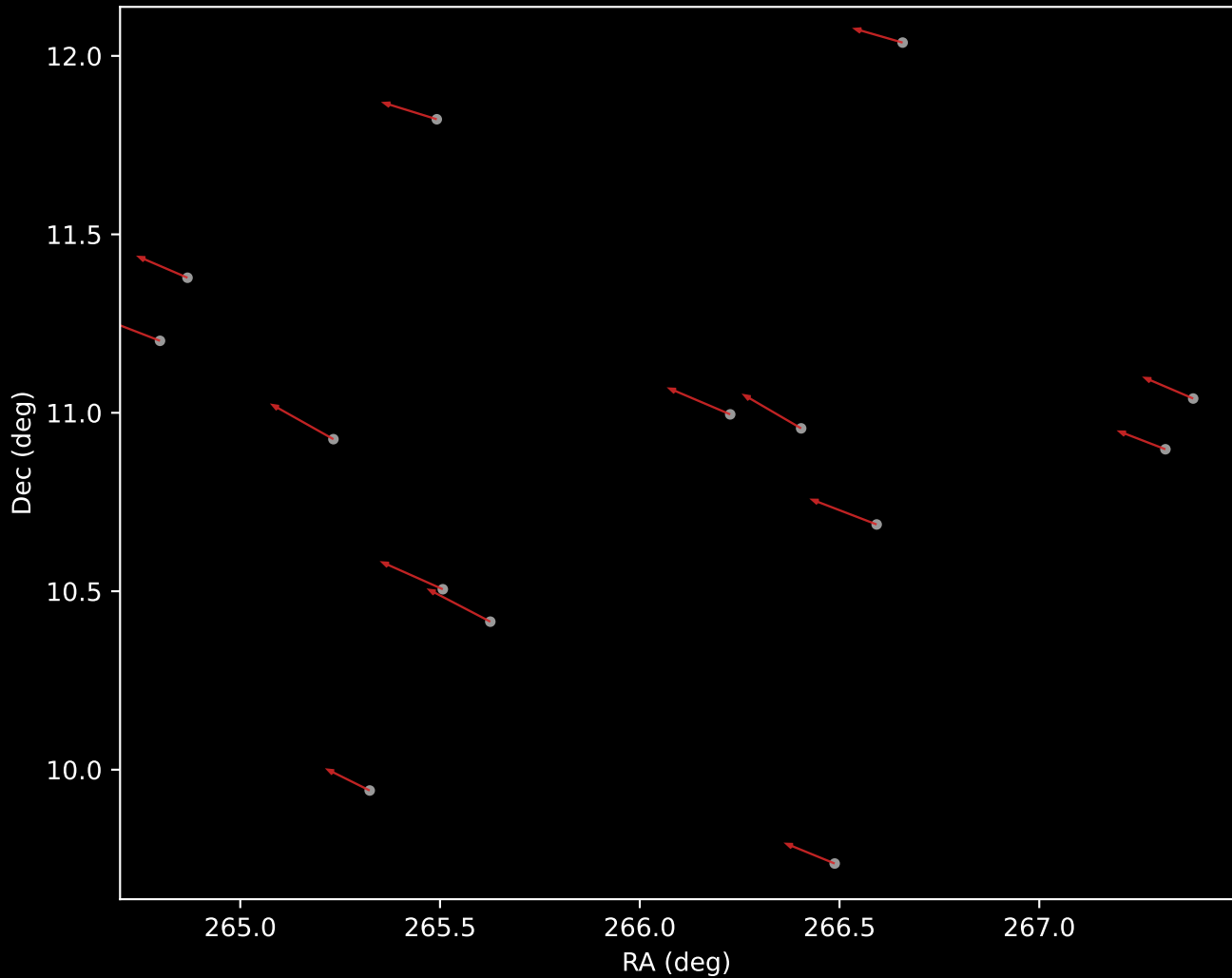
APOGEE DR17 Cluster 6 Proper Motion Vectors (n=14)
