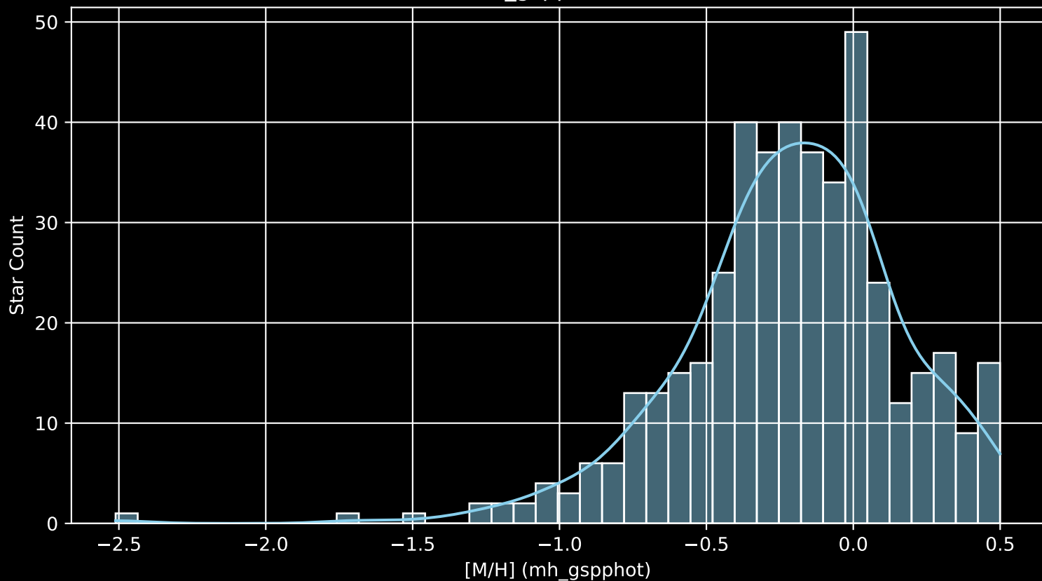
APOGEE DR17 Field: [240+60 [M/H] (mh_gspphot) (n= 440)
