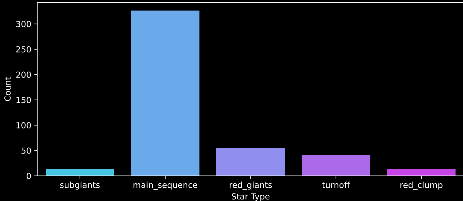
APOGEE DR17 Field: [240+60] Count plot of Star Type
